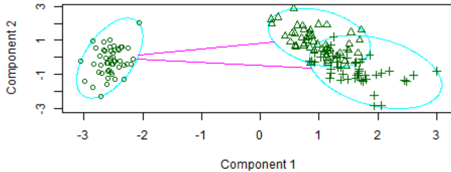
clusplot(clara(x = transit, k = 3))
