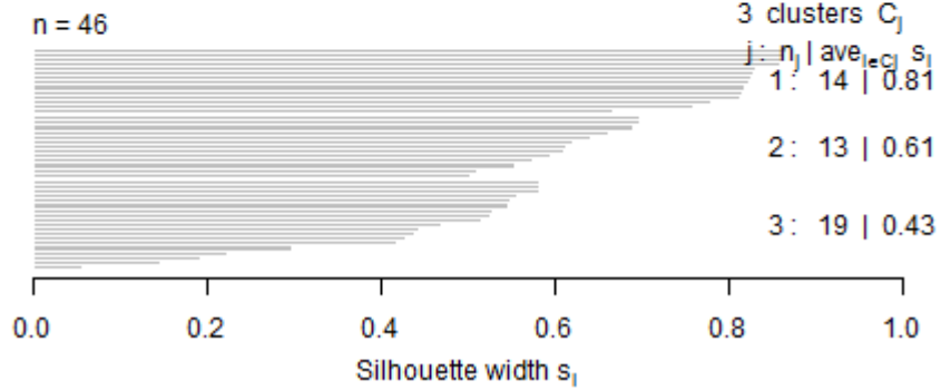
Silhouette plot of clara(x = transit, k = 3)
